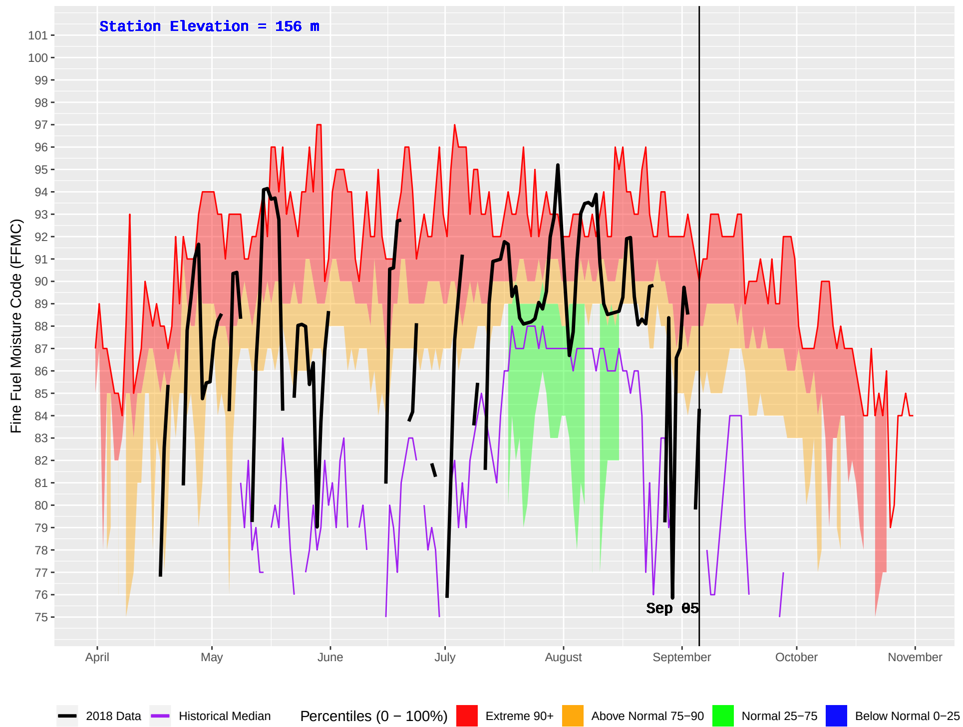
WOSS CAMP (21) : Historical (1970–2016) and Current (2018) Daily Fine Fuel Moisture Code (FFMC)
