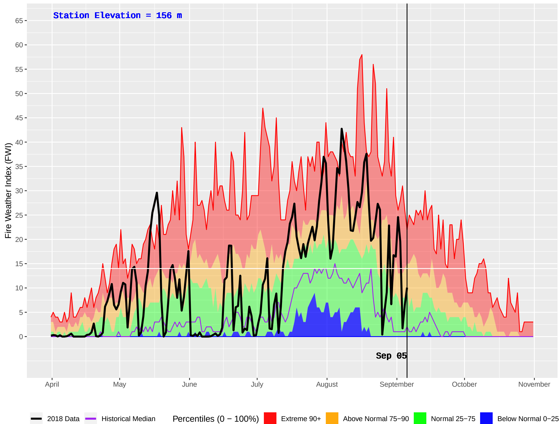
WOSS CAMP (21) : Historical (1970–2016) and Current (2018) Daily Fire Weather Index (FWI)
